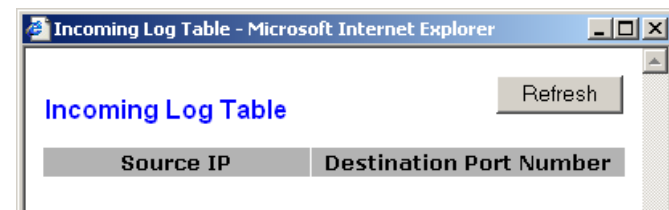
Figure 5-31: Log Table
