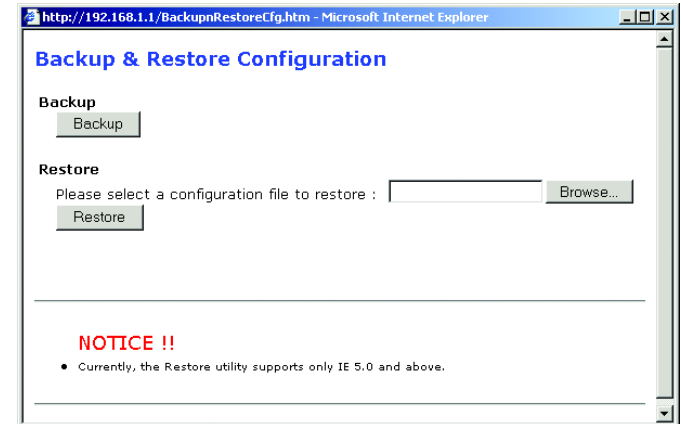
Figure 5-29: Backup & Restore
