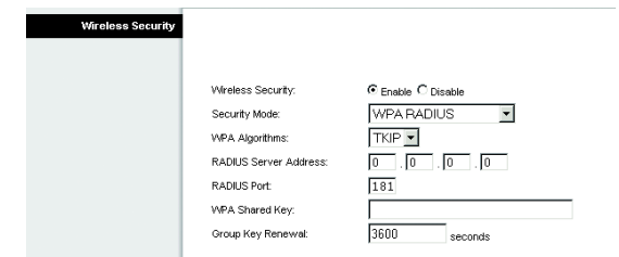
Figure 5-15: WPA Radius
